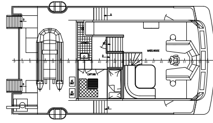
Wheelhouse deck
